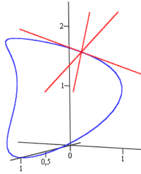
Rectas tangente, normal principal y normal
